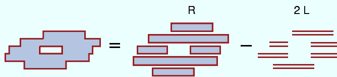
Fig. 2. The perimeter of a run-length encoded bitmap is easily computed by adding the perimeters of each horizontal run and subtracting twice the length of the contact segments between runs located on adjacent rows.
